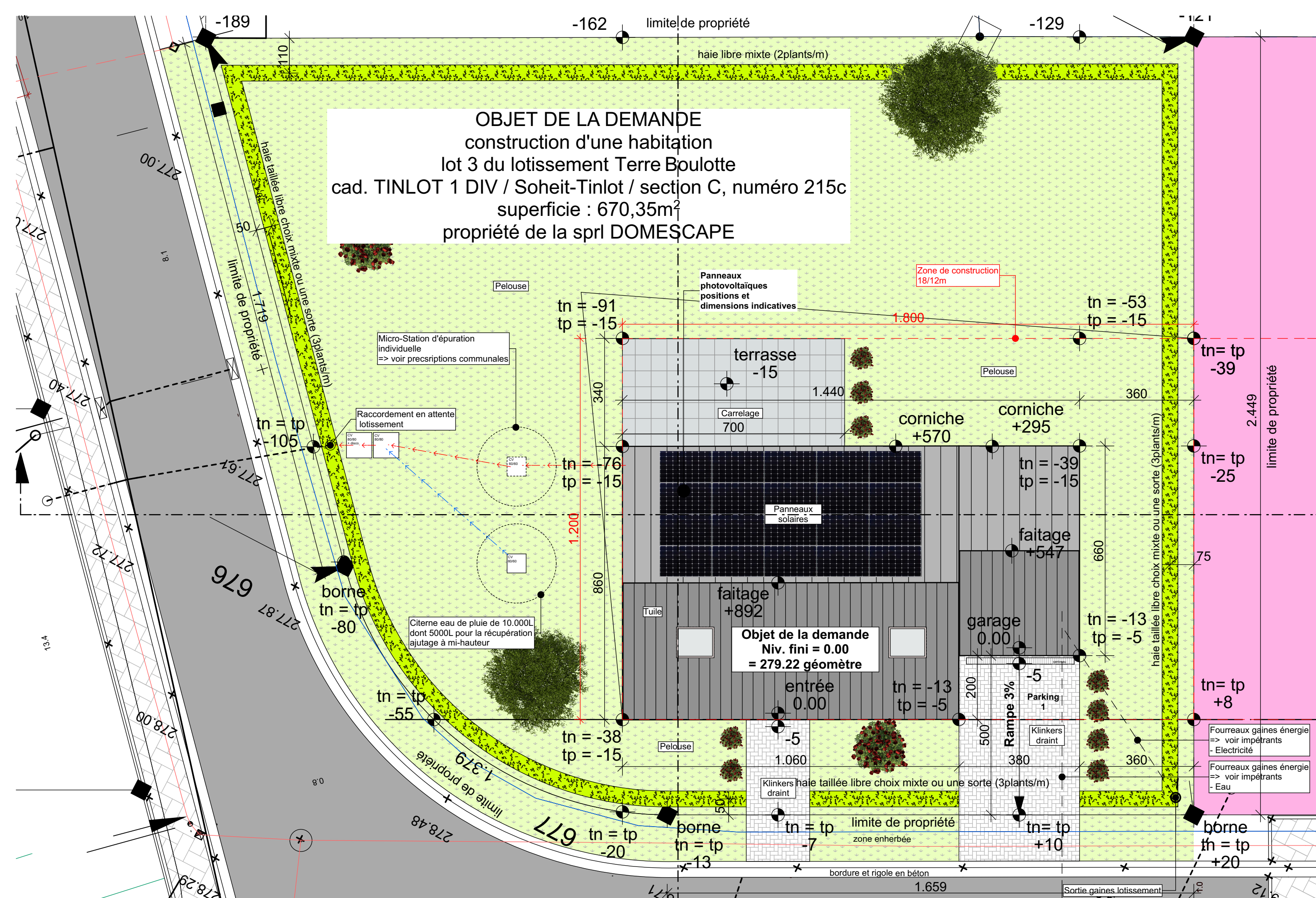
Implantation 1/100
