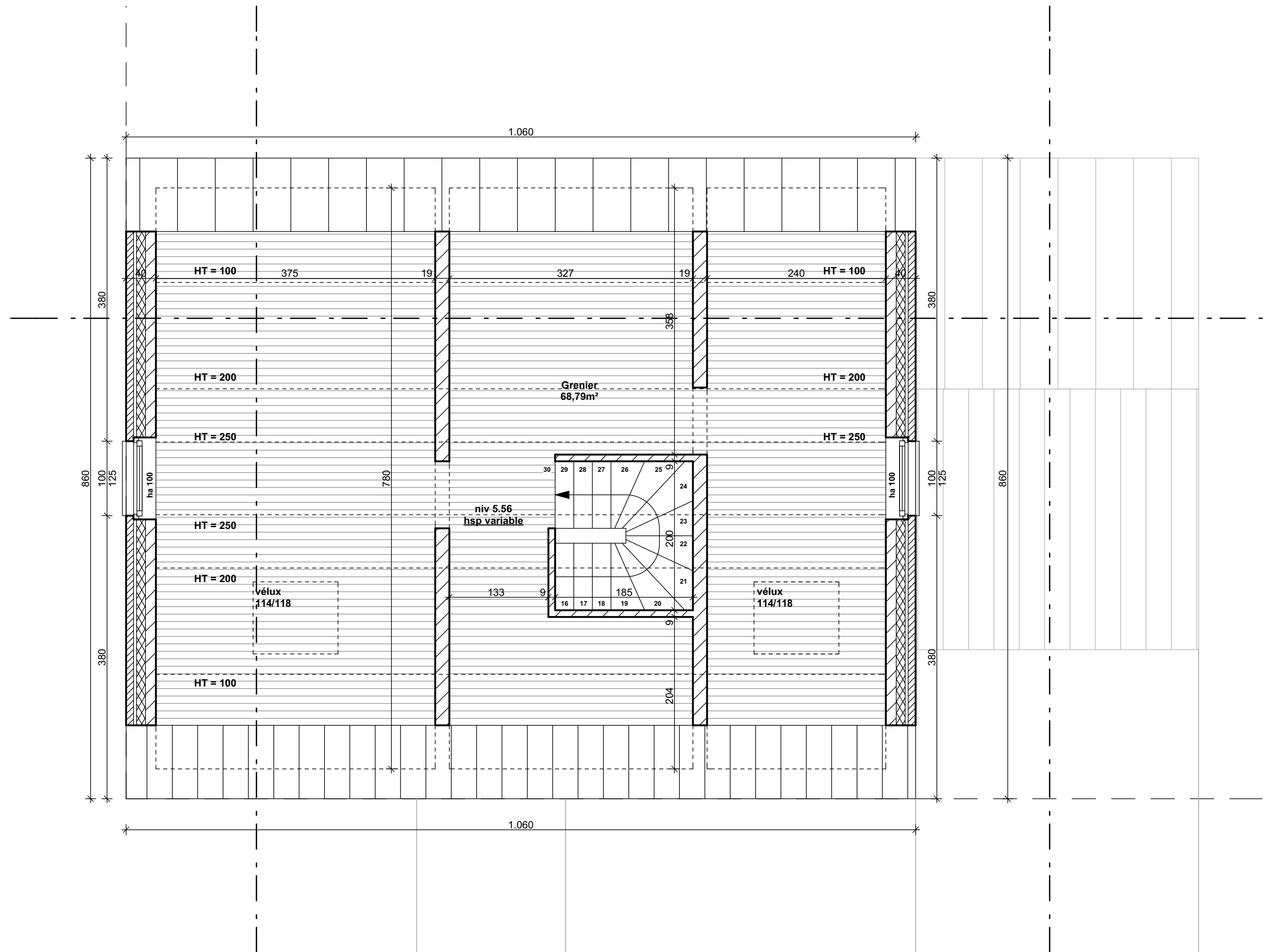
Plan grenier 1/50
